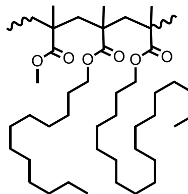
Polymethacrylate (PMA) Mixture of short, medium, and long fatty esters; medium to high MW
